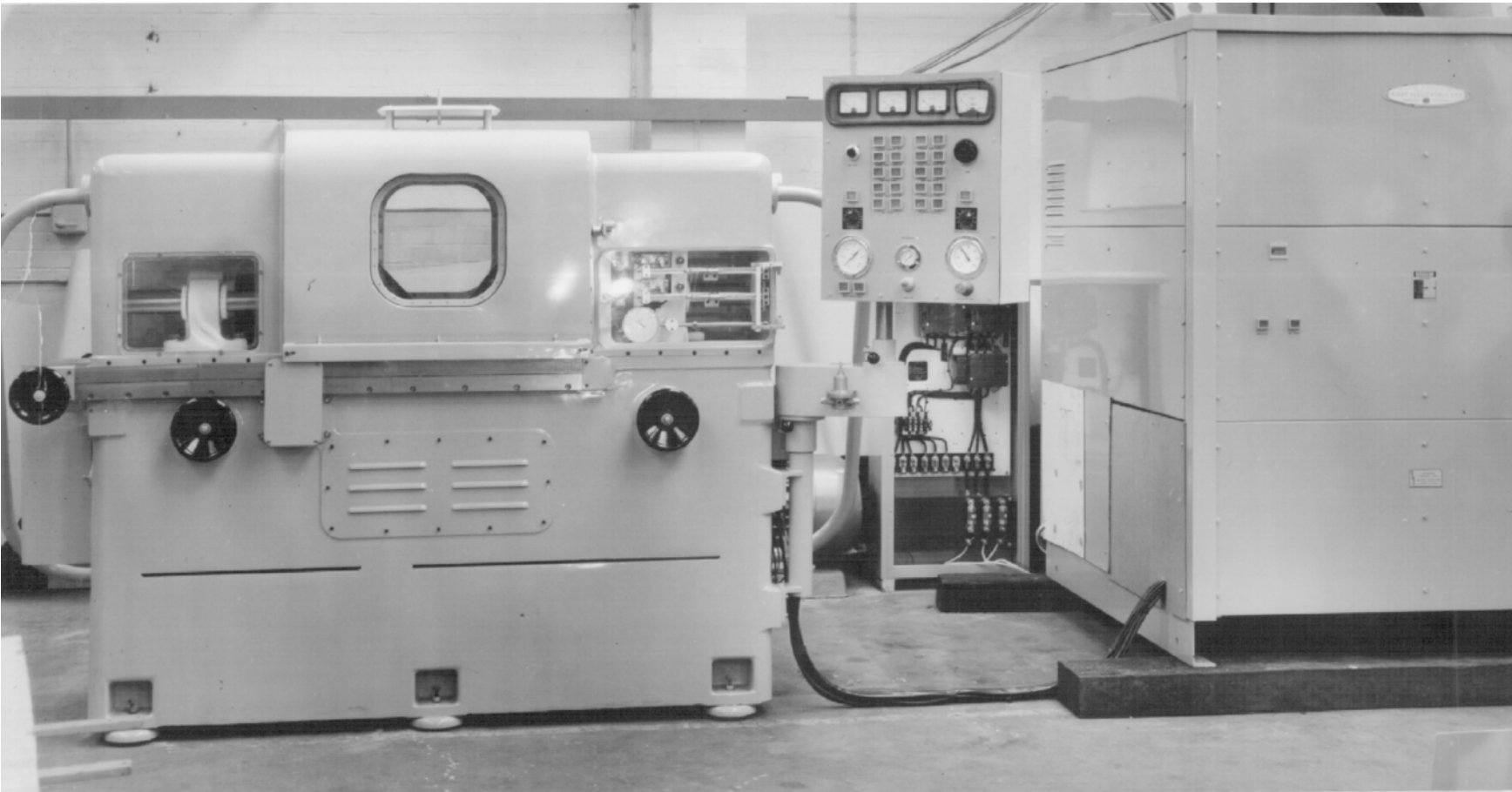
Twin Ram Electro Chemical Machine for Blade Aerofoils ( Rolls-Royce )
